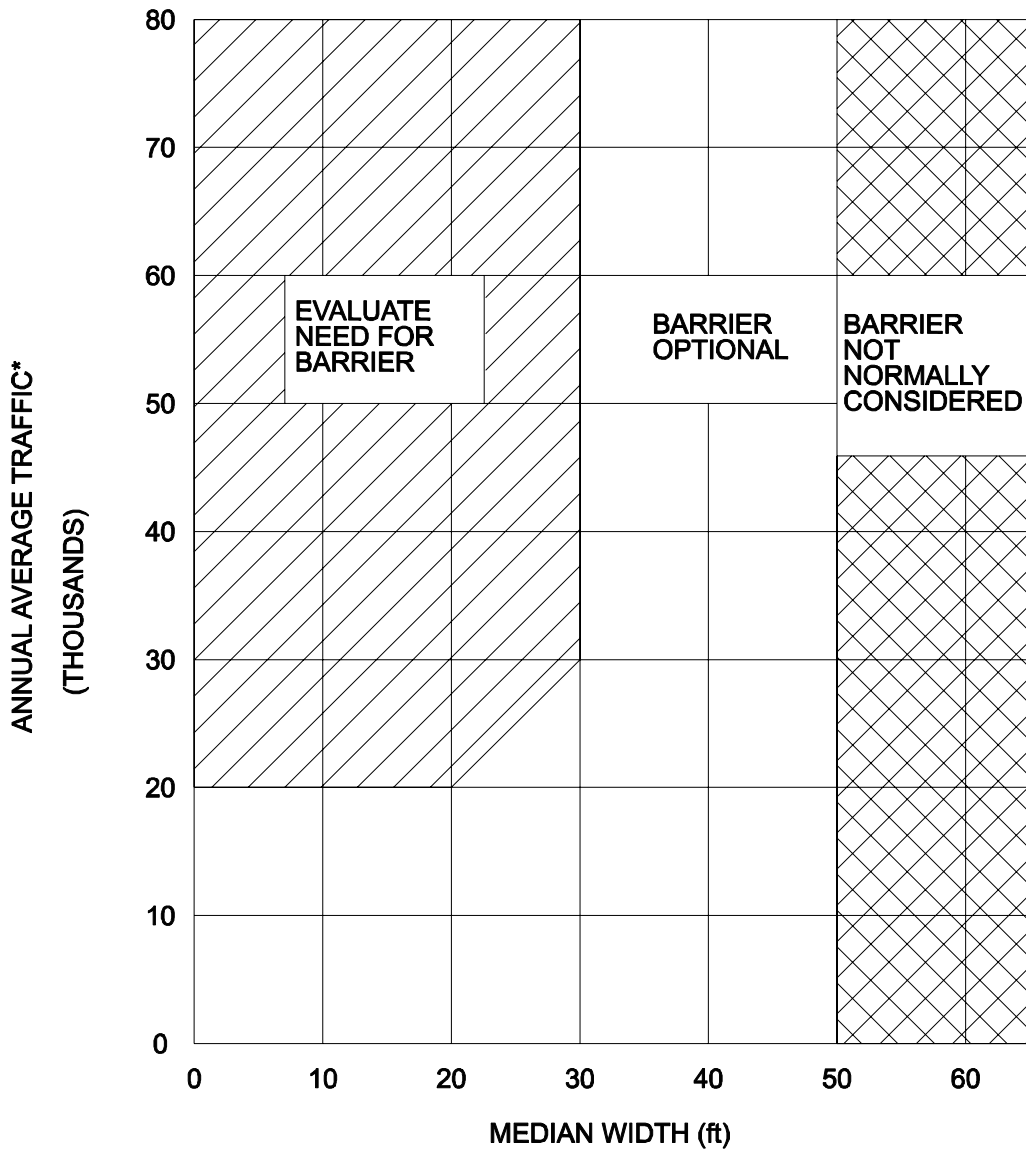
* BASED ON A MINIMUM FIVE-YEAR PROJECTION MEDIAN BARRIER WARRANTS Figure 14.5A (Metric)
