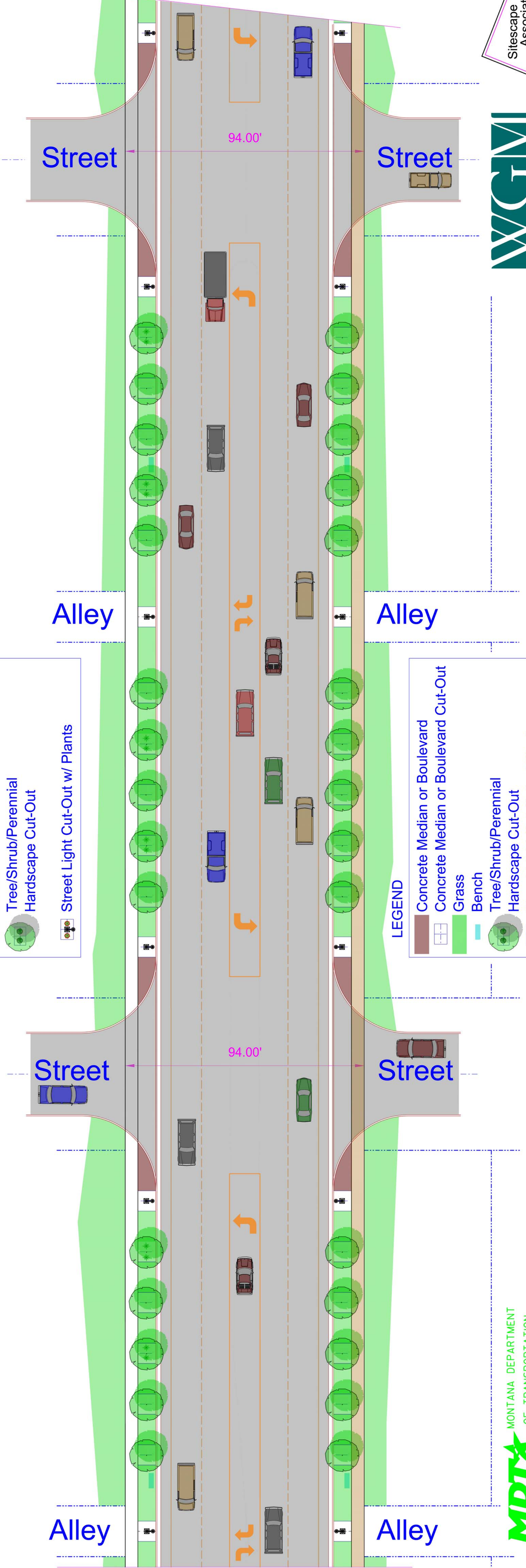
TYPICAL PLAN NO.2
