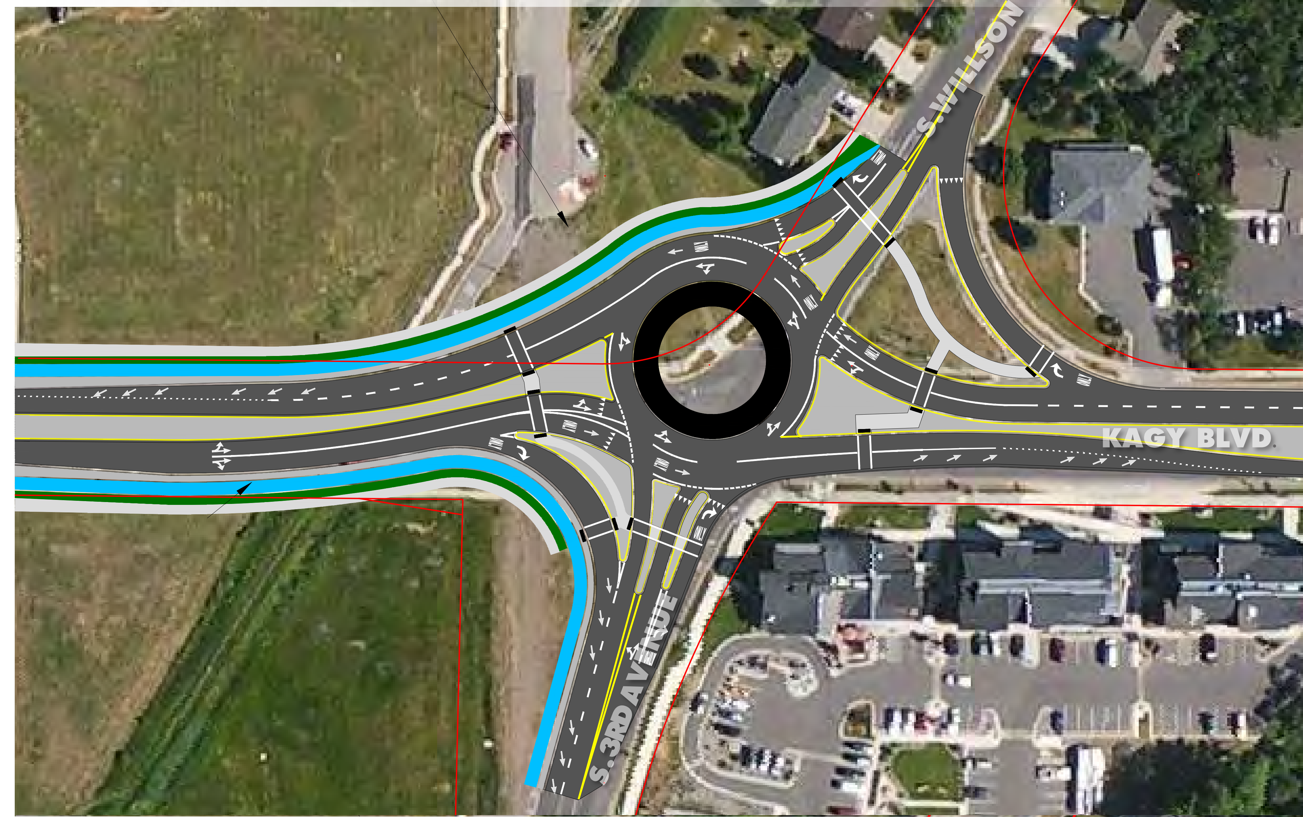
MULTI-LANE ROUNDABOUT
