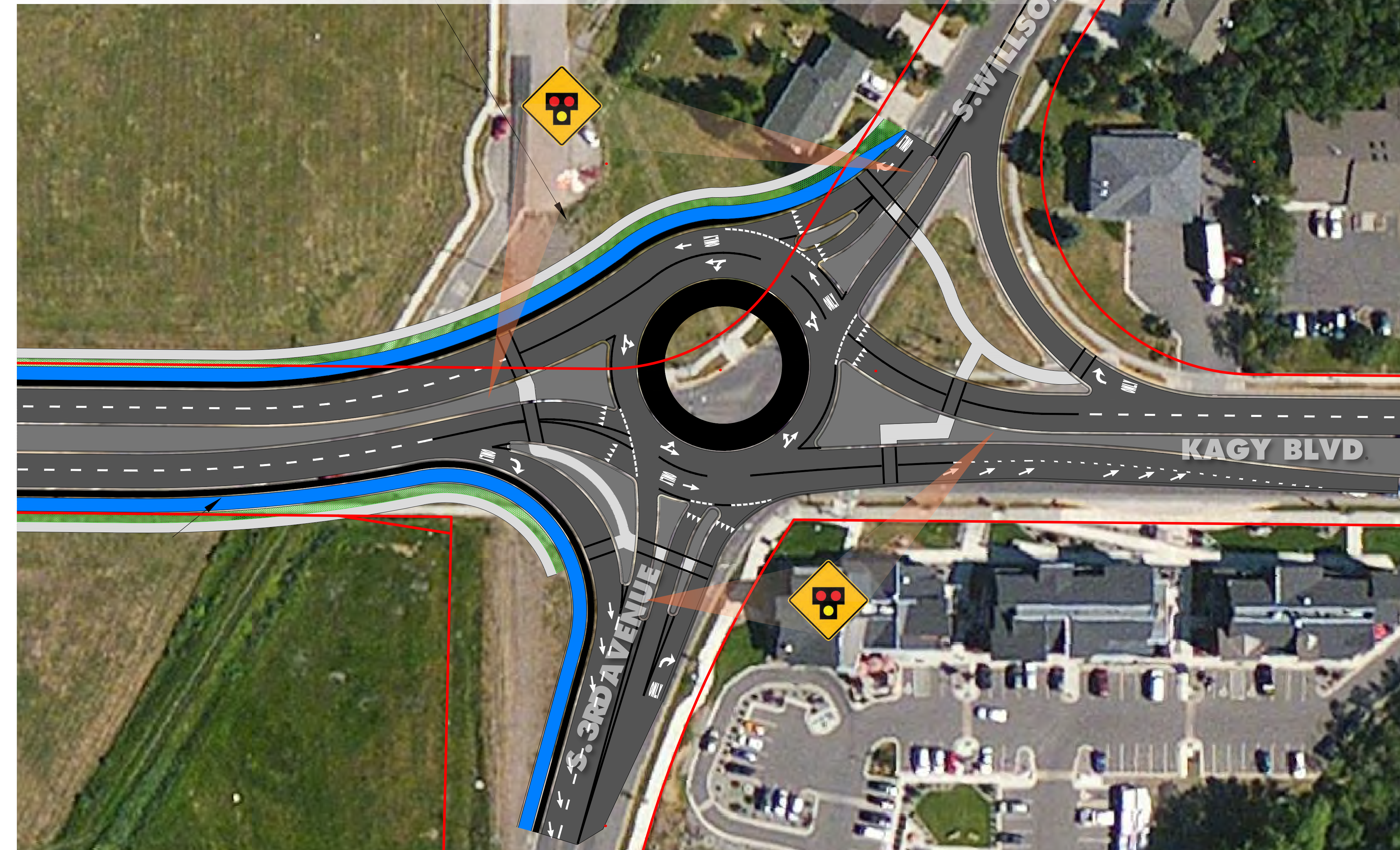
MULTI-LANE ROUNDABOUT
