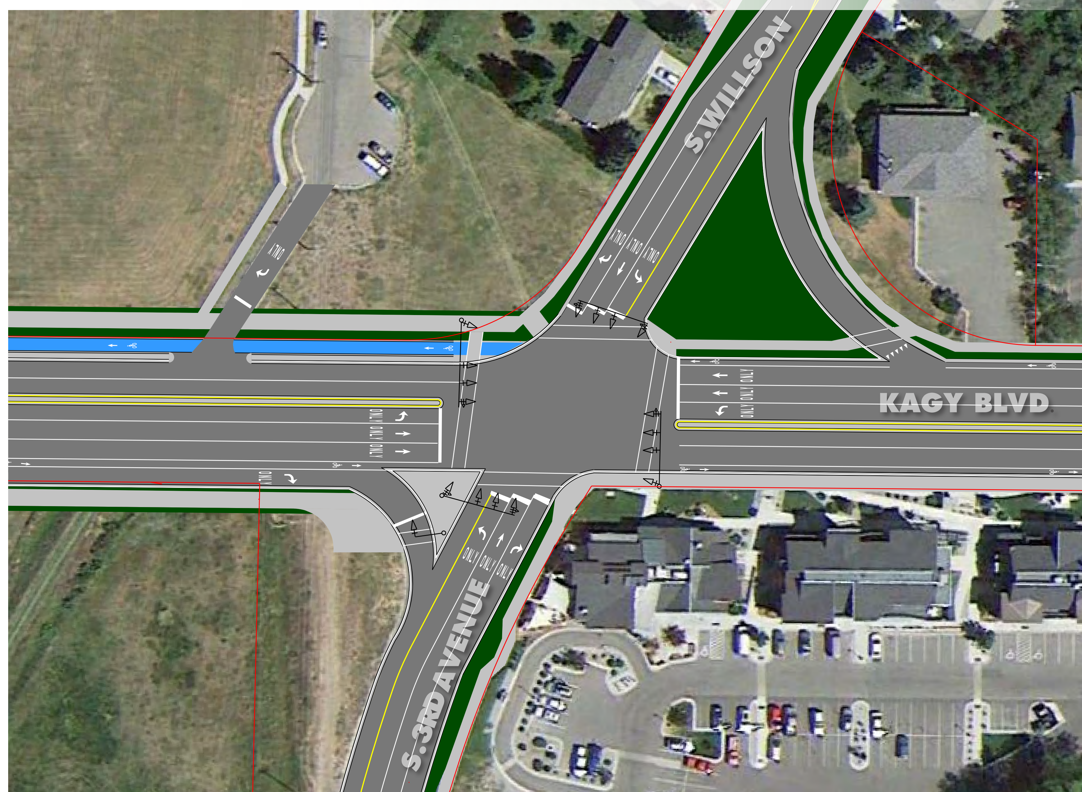
MULTI-LANE SIGNALIZED INTERSECTION
