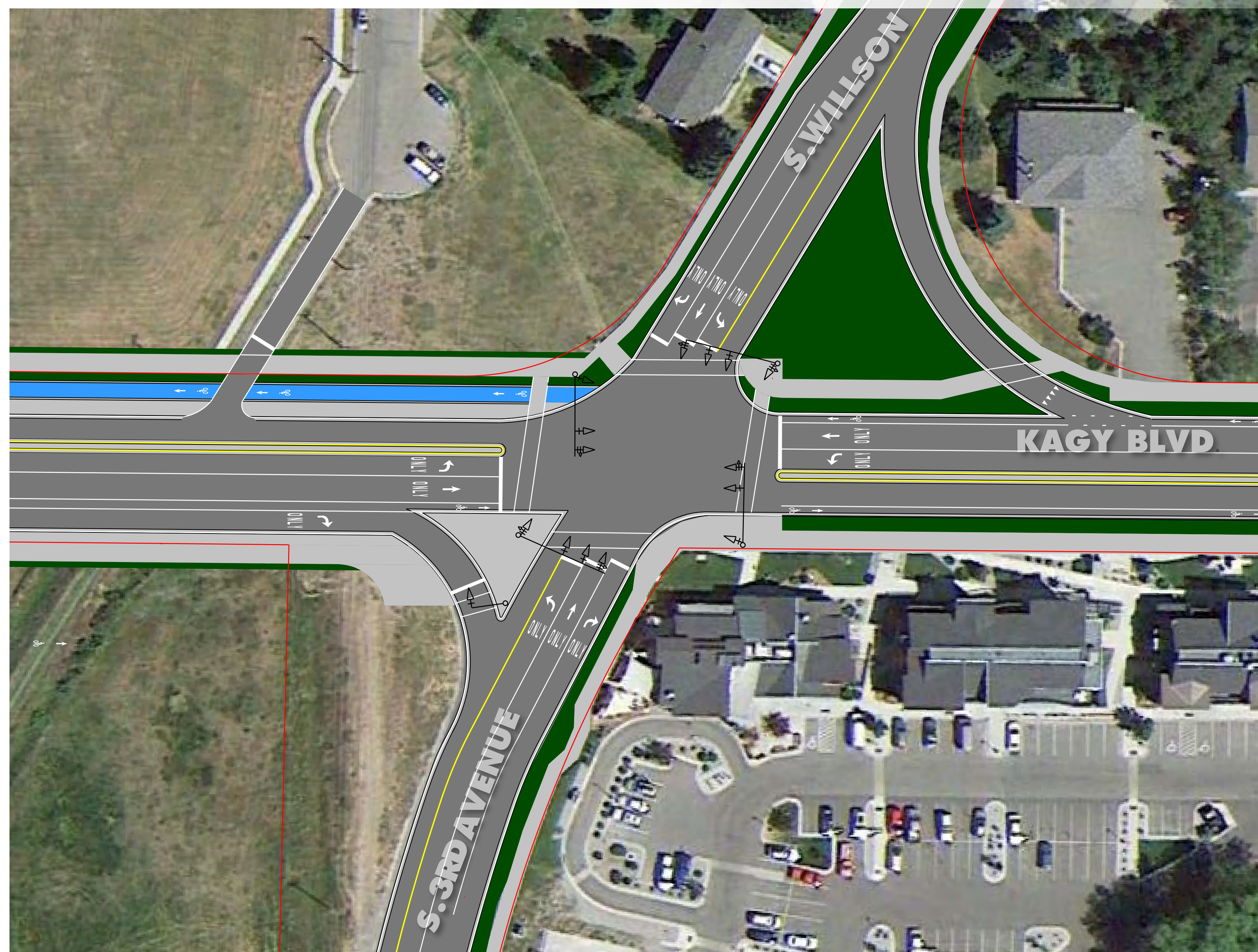
MULTI-LANE SIGNALIZED INTERSECTION
