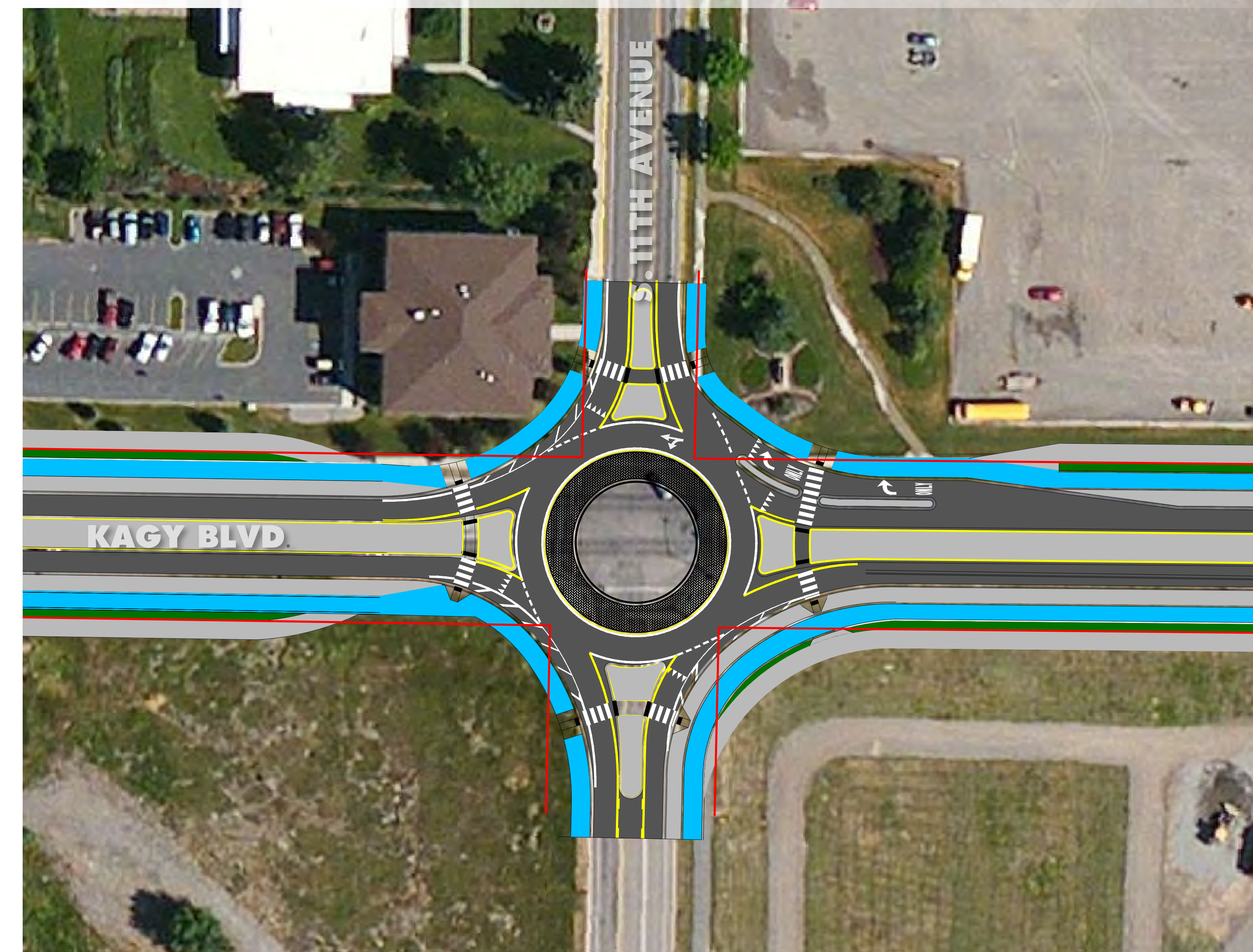
MULTI-LANE ROUNDABOUT
