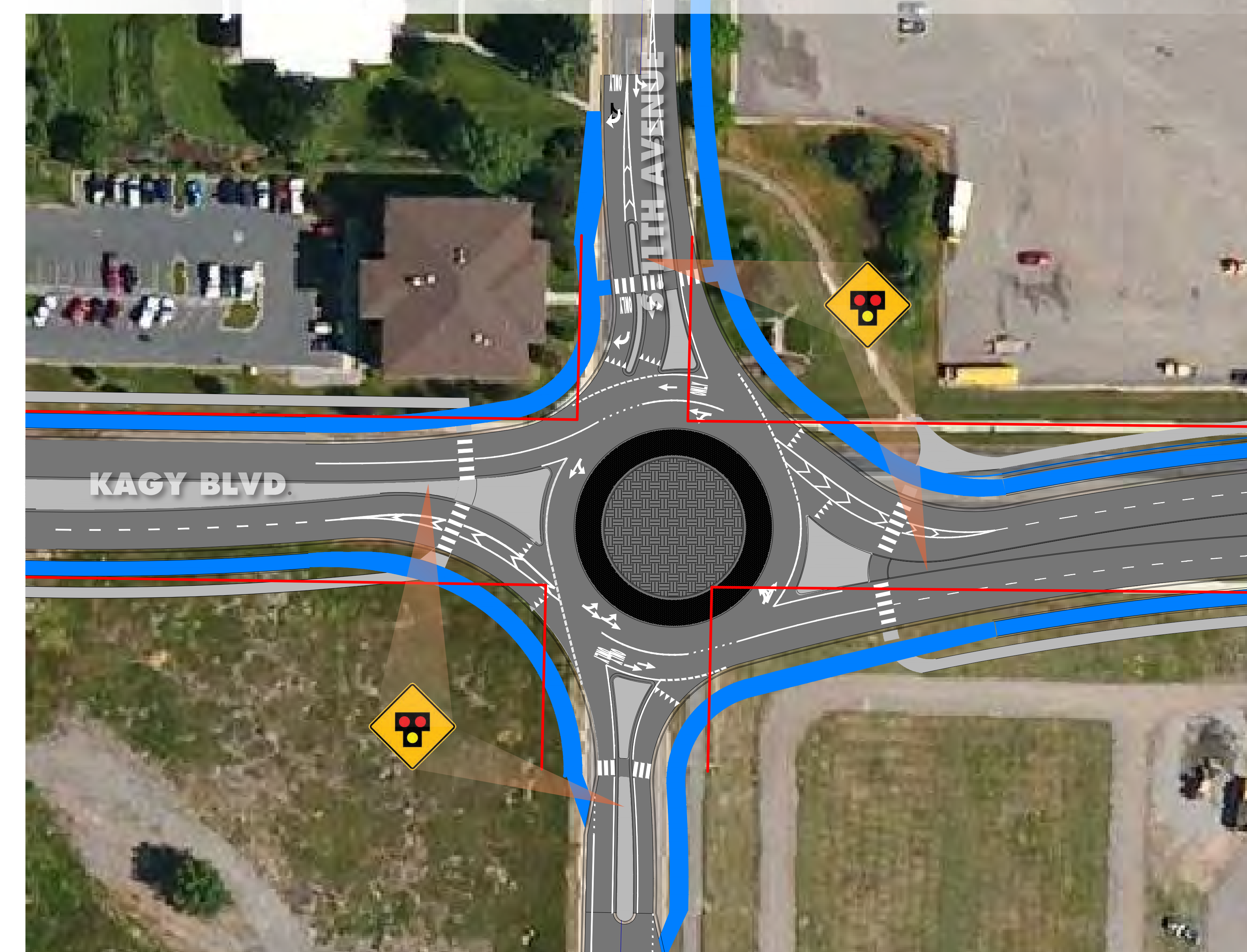
MULTI-LANE ROUNDABOUT
