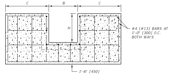
SECTION E-E
