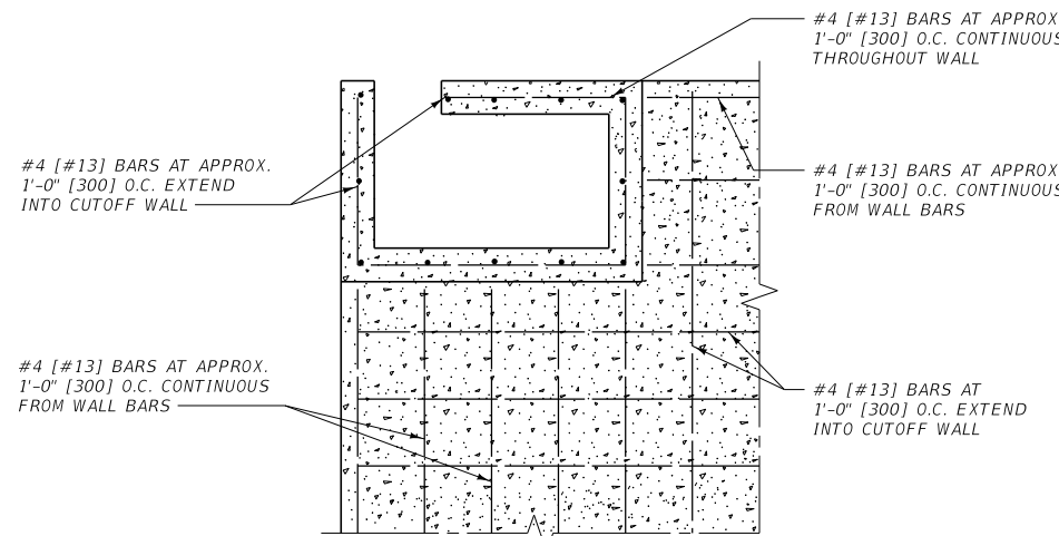
SECTION F-F
