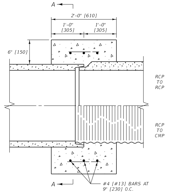
CONNECTION DETAILS
