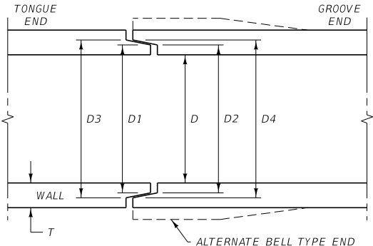
JOINT DETAIL
