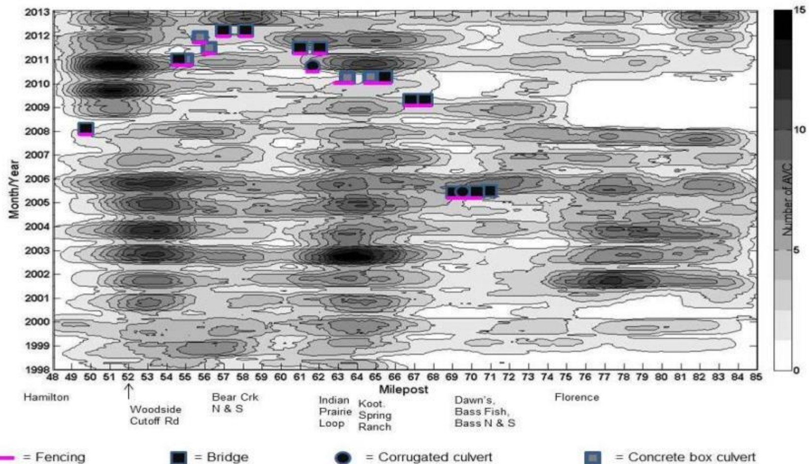
Figure 2. Kernel Density Analysis of AVC carcass data, US 93 South, mp 48 through 85, 1998 to 2013. Darker spots reflect higher carcass counts at specific mile posts. Wildlife crossing structure type, location, date installed, and wildlife fencing are indicated. Wildlife crossing structure icons are not to scale of graph.
