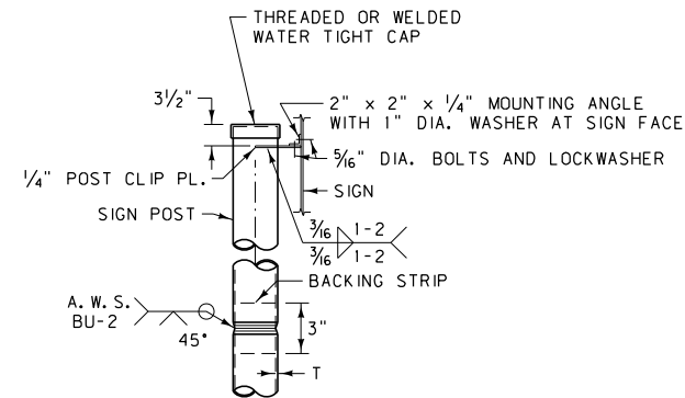
TYPICAL SPLICE
