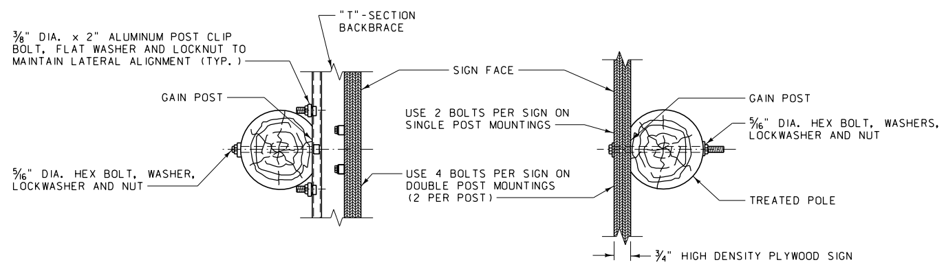
TREATED POLE SINGLE OR DOUBLE (USED WHEN "T"-BAR WIND BEAMS NOT REQUIRED)
