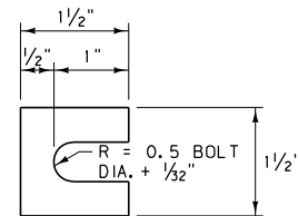
SHIM DETAIL
